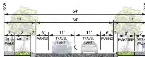
Local Street – 48' ROW
