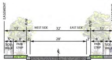
Sub Local Street – 32' ROW (13' Easement on each side) (For roadways with a projected ADT of 800 or less)
