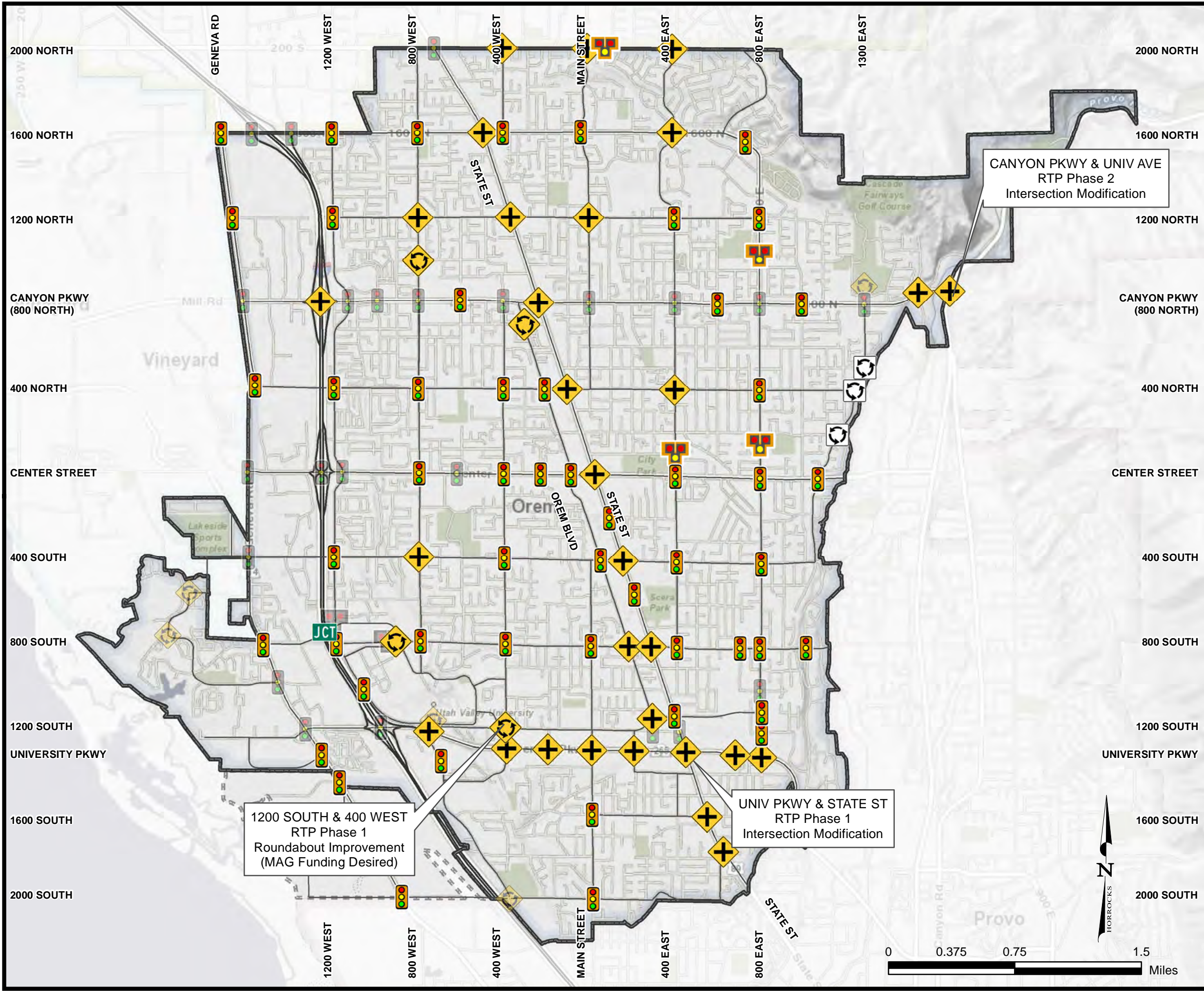
Figure 25: 2040 Intersection Improvements
